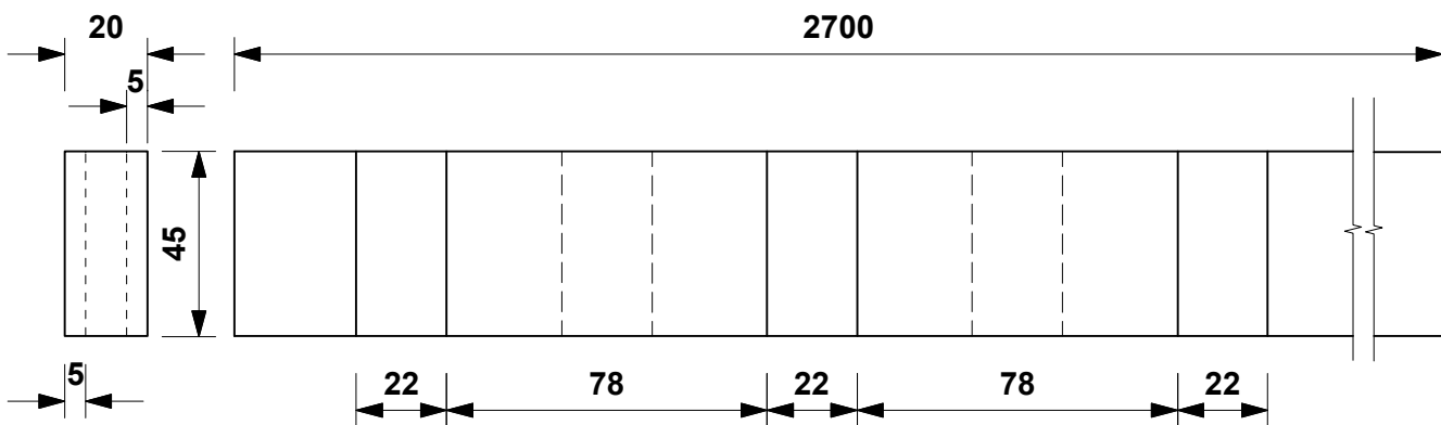
TOP VIEW
