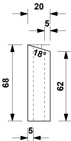
END VIEW
