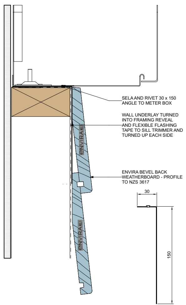
FLASHING DIMENSIONS
