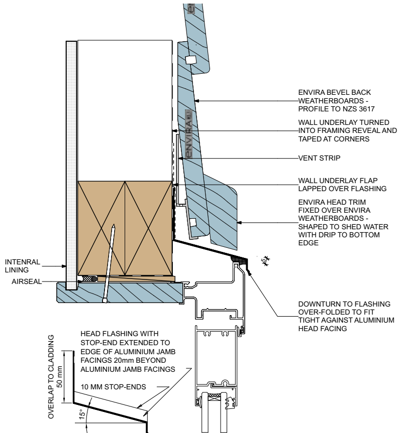
FLASHING DIMENSIONS
