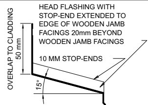
FLASHING DIMENSIONS
