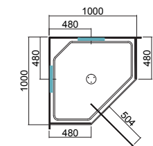
1000 x 1000
