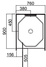
900 x 760 (760 door)
