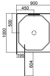
1000 x 900 (900 door)
