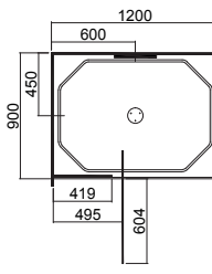
1200 x 900 (1200 Door)
