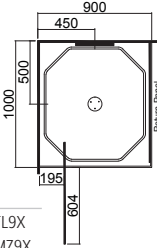
1000 x 900 (900 door)
