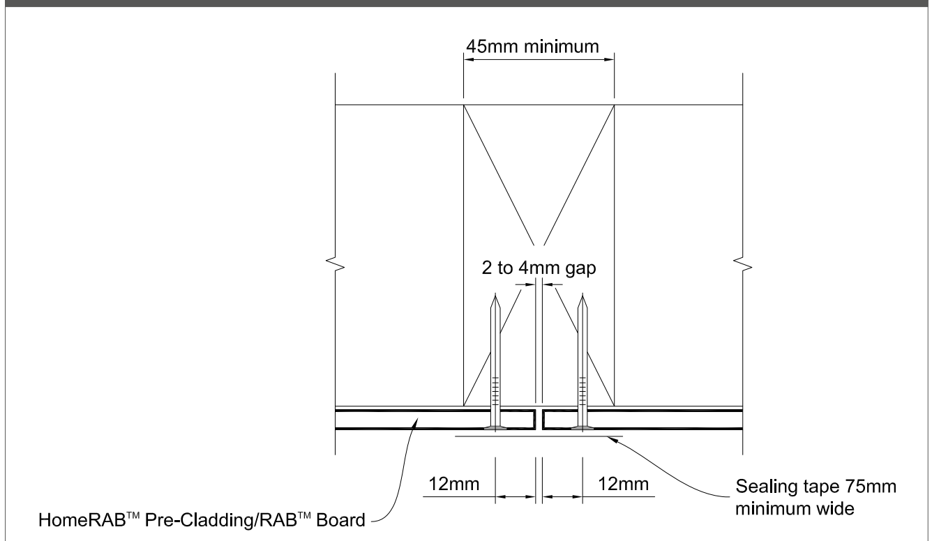
Figure 7: Vertical joint
