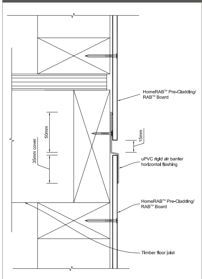
Figure 9: Horizontal joint/flashing - floor joist
