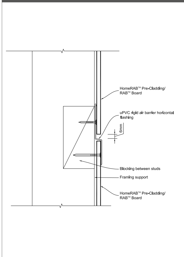
Figure 8: Horizontal joint flashing - tall wall
