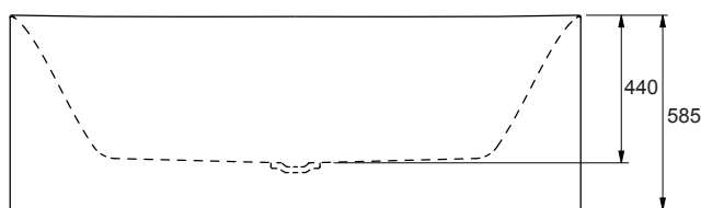
1700 Freestanding BTW/Corner Bath - Front View
