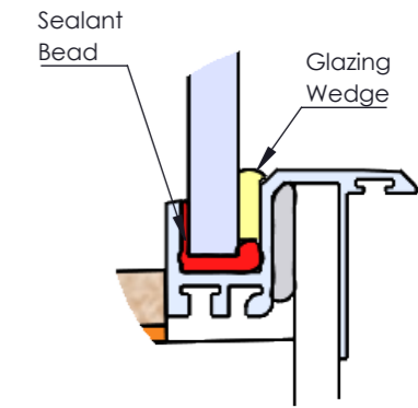
Glass Panel Silicone Detail DETAIL D
