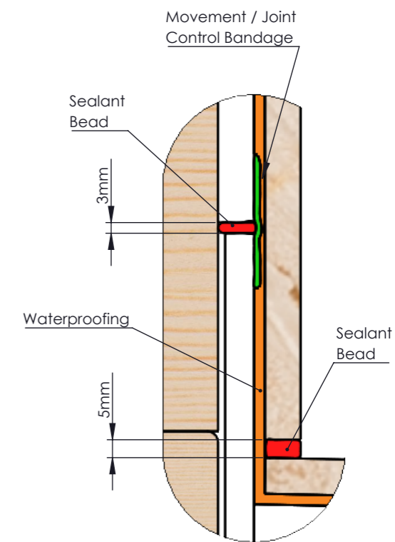
Wall Joint Detail DETAIL C
