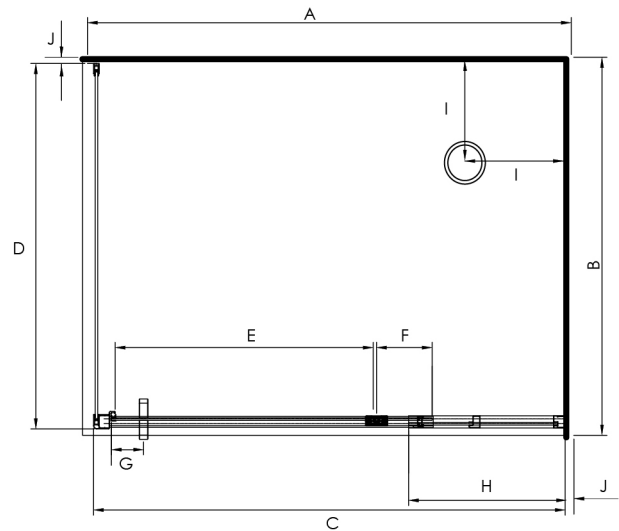
Dimension drawing depicts - Aquero Pivot Door RH .
