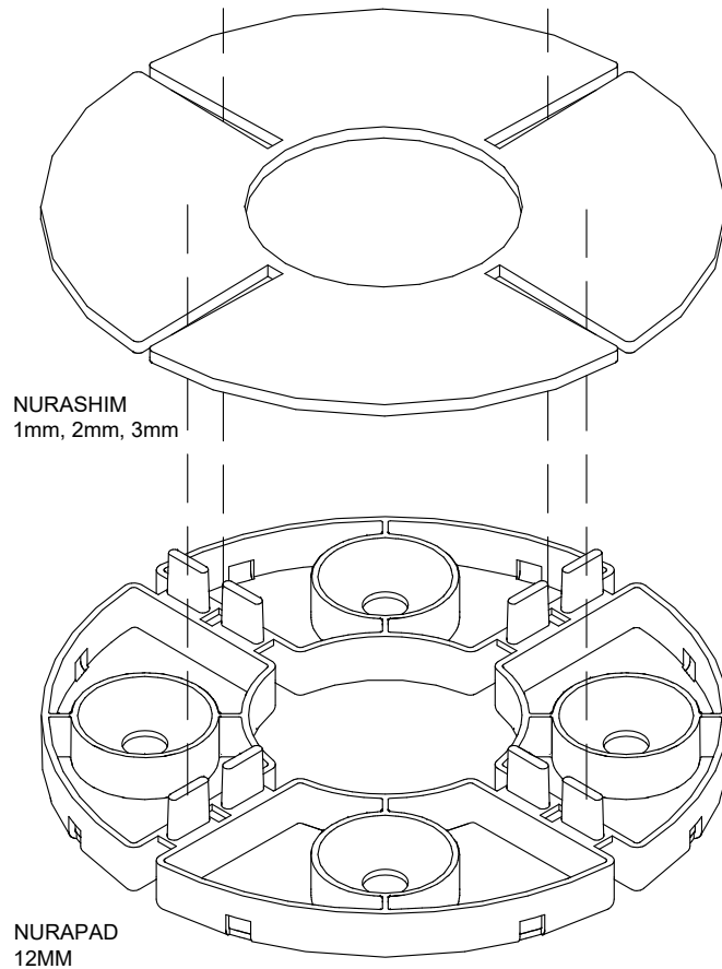
ISOMETRIC
